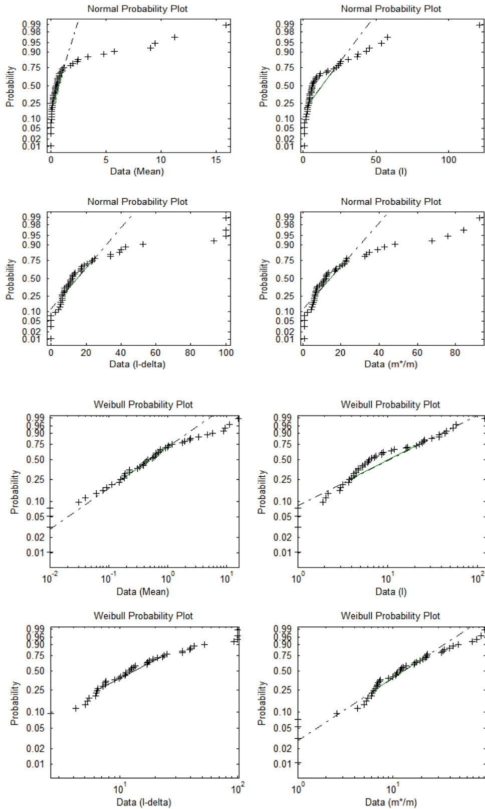
Fig. 3 Fitting goodness of the mean, l , l_{\delta} , m^*/m with normal distribution and Weibull distribution. Linear relationship between probability and data means that the mean and three indices follow Weibull distribution rather than normal distribution.
