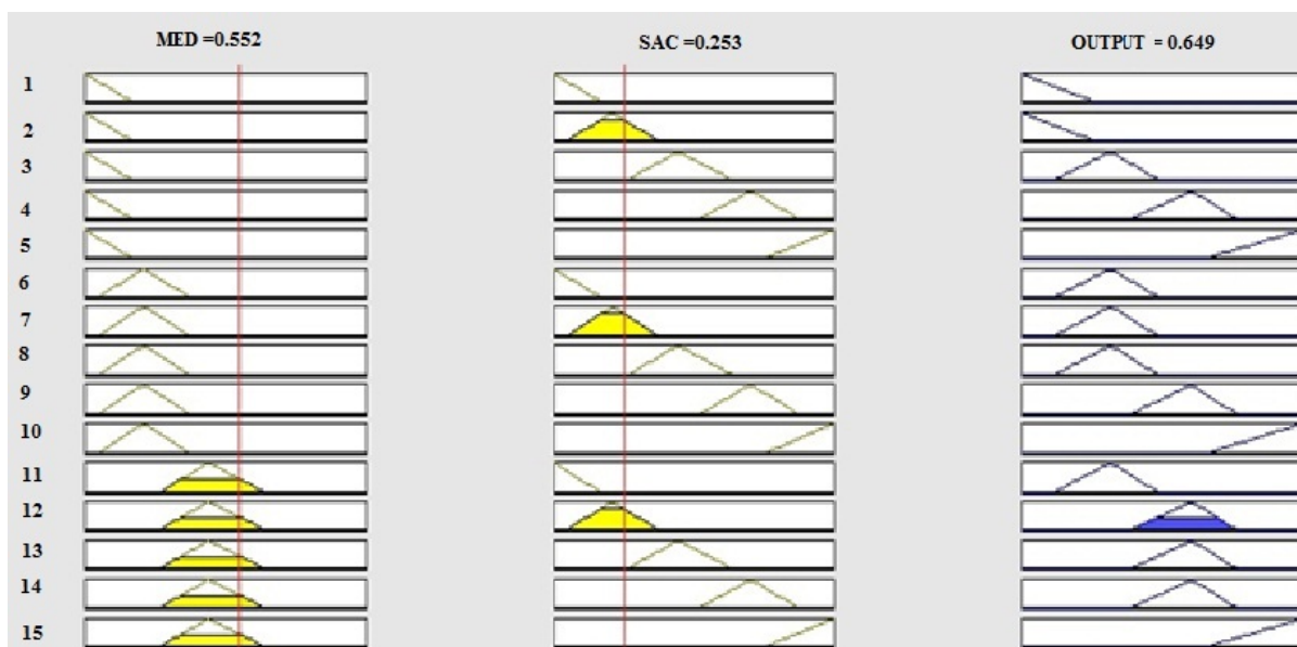
Fig. 4 The rules which are used for a fuzzy combination of the (MED ij ) and (SAC ij ) criteria.
